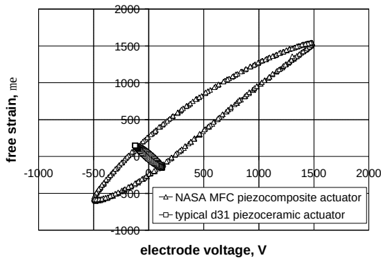
Figure 4. LaRC-MFC piezocomposite longitudinal (fiber-direction) free-strain actuation behavior.
