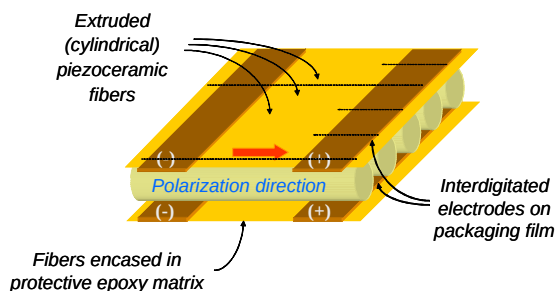
Figure 1. First generation piezocomposite actuator concept.
