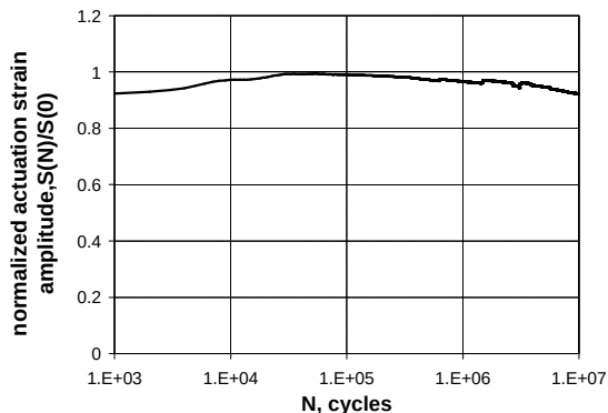
Figure 9. Strain actuation trends under 1000 microstrain static load at elevated temperature (65C, 1000Vp-p, 100 Hz).
